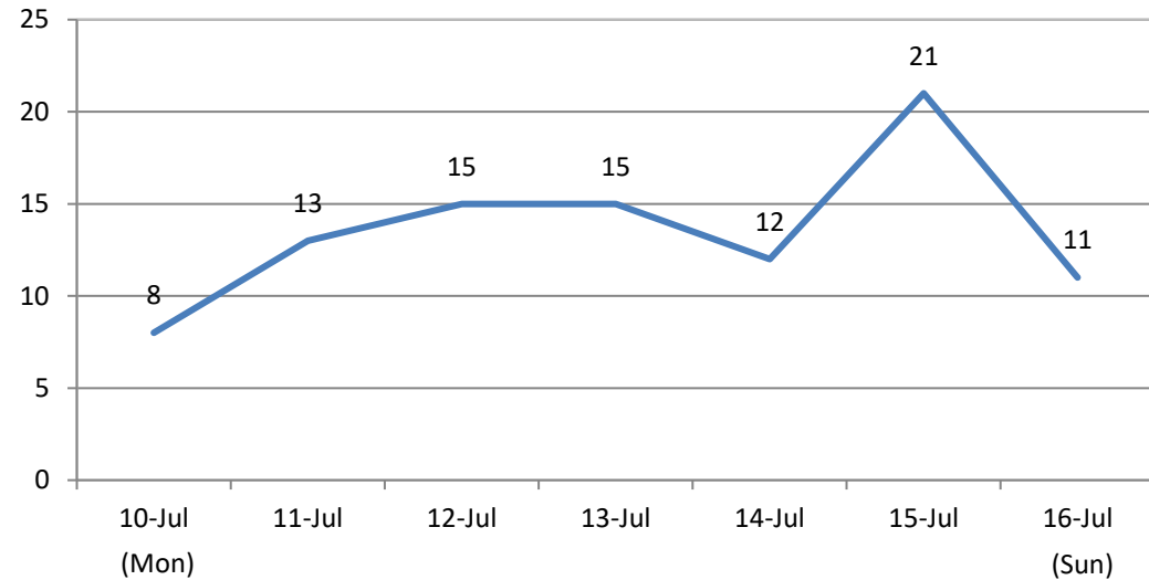
Est. ED Visits Due to Drug Overdoses by Day, Jul 10 - Jul 16, 2017
